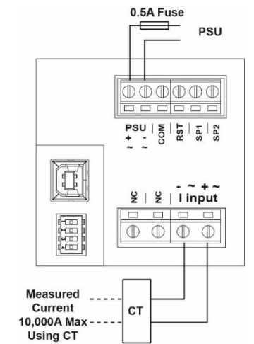
AMMETER USING CURRENT TRANSFORMER
