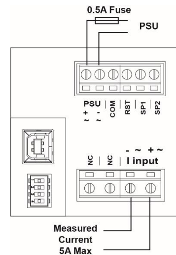
AMMETER DIRECT
