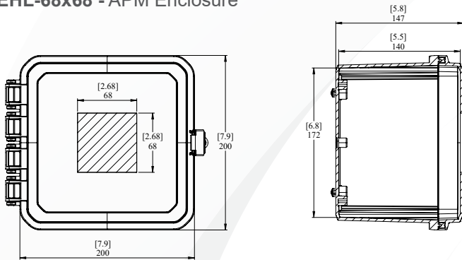
EHL-68x68 - APM Enclosure
