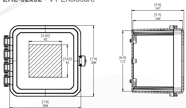
EHL-92x92 - VT Enclosure
