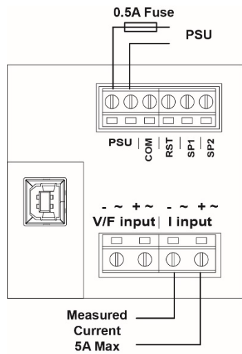
AMMETER DIRECT
