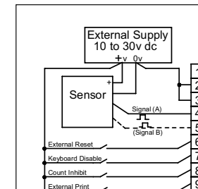
Illustrating use of external power supply (source mode depicted).
