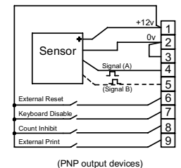
(PNP output devices)
