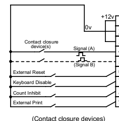
(Contact closure devices)
